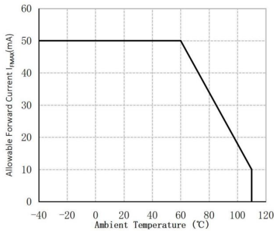
Fig.1 Allowable Forward Current VS Ambient Temperature
