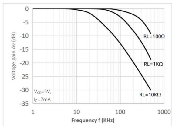
Fig.10 Frequency Response
