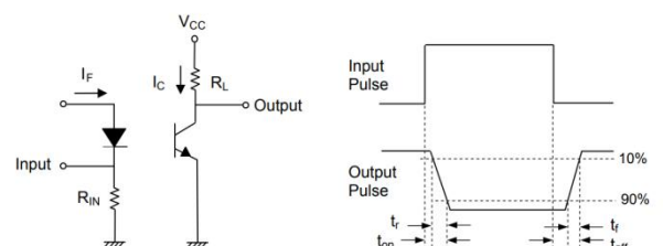
Fig.12 Switching Time Test Circuit & Waveforms
